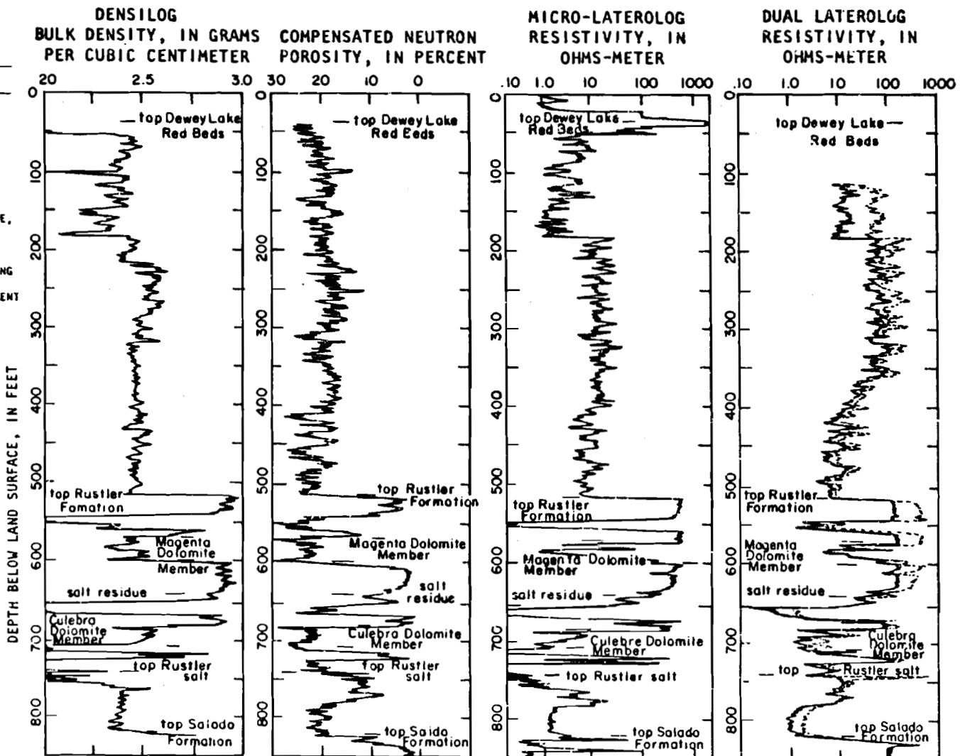
Figure 3.--Selected geophysical logs for well H-1.
