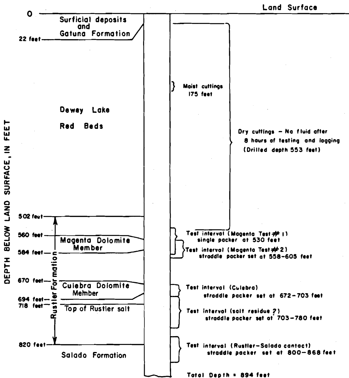
Figure 9.--Open-hole intervals tested in well H-3.
