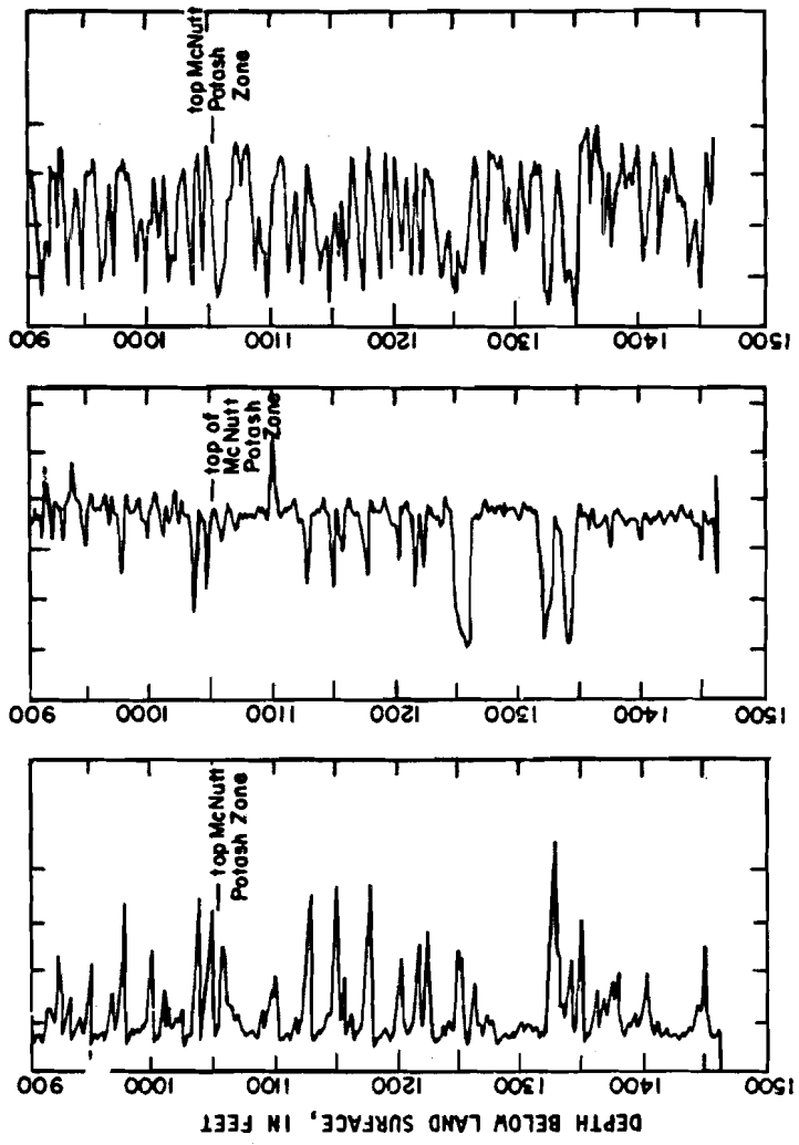
Figure 17.--Selected geophysical logs for well P-15.
