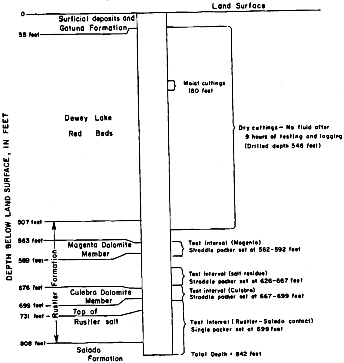
Figure 5.--Open-hole intervals tested in well H-1.
