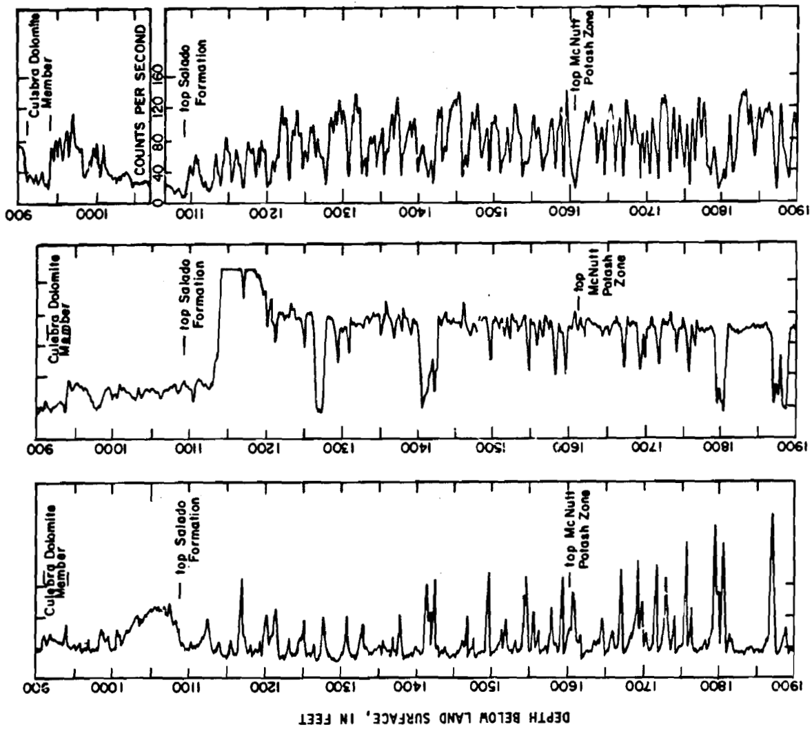
Figure 21.--Selected geophysical logs for well P-18.
