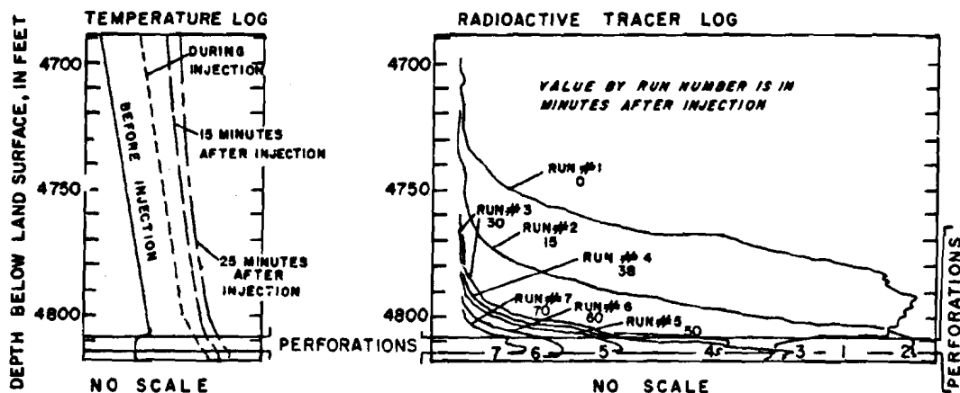
Figure 26.--Radioactive tracer (tracejector) and temperature logs in the Bell Canyon Formation for well AEC-8.
