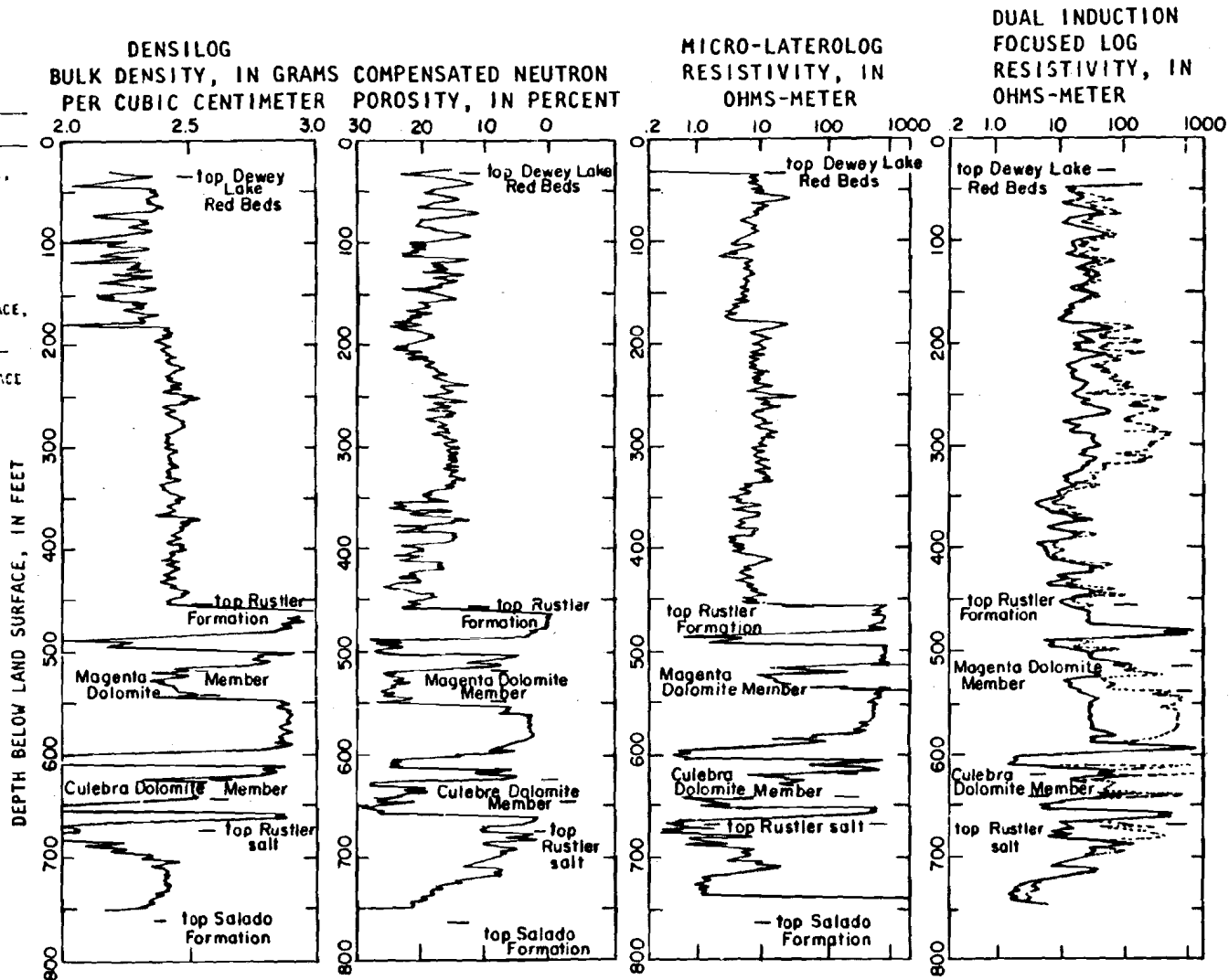
Figure 11. Selected geophysical logs for well H-2c.
