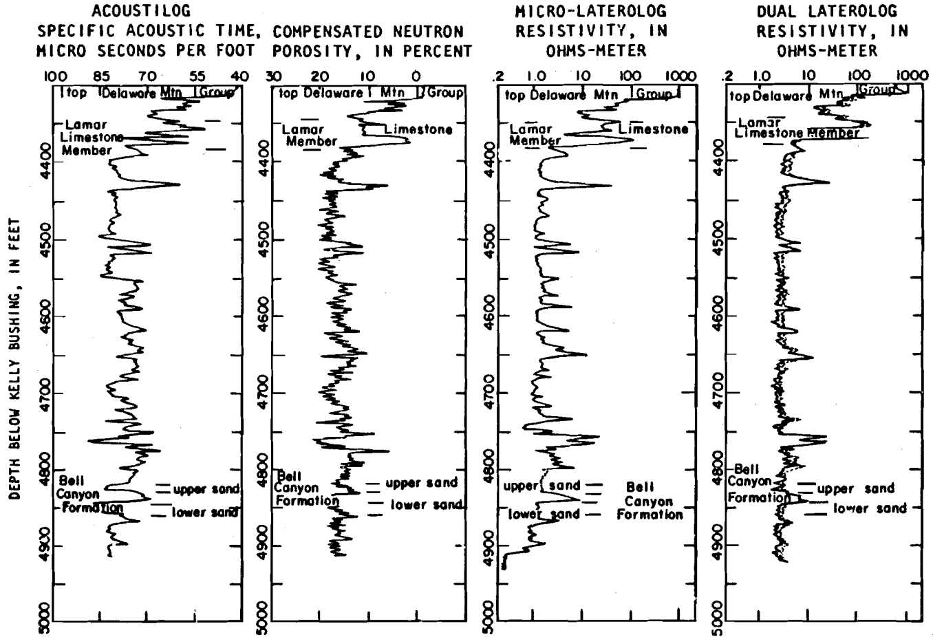
Figure 23.--Selected geophysical logs for well AEC-8 -Concluded.
